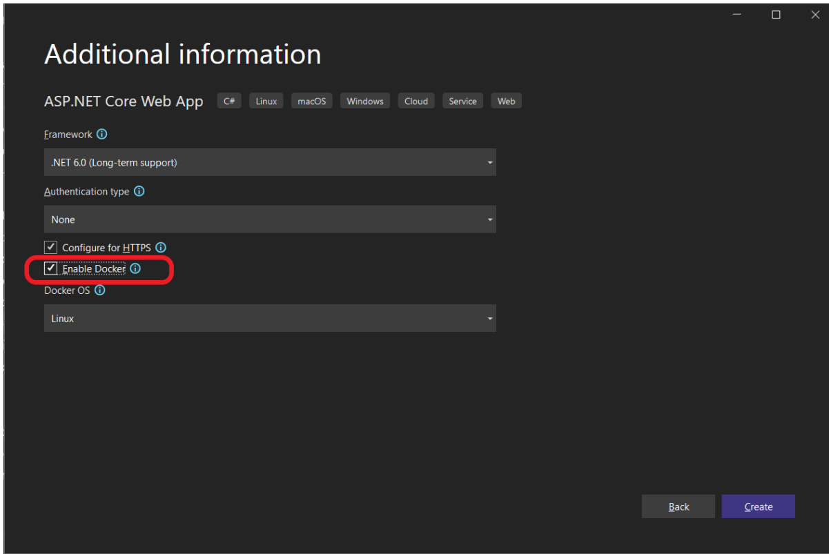
Figure 4-32. Enable Docker support during project creation in Visual Studio
