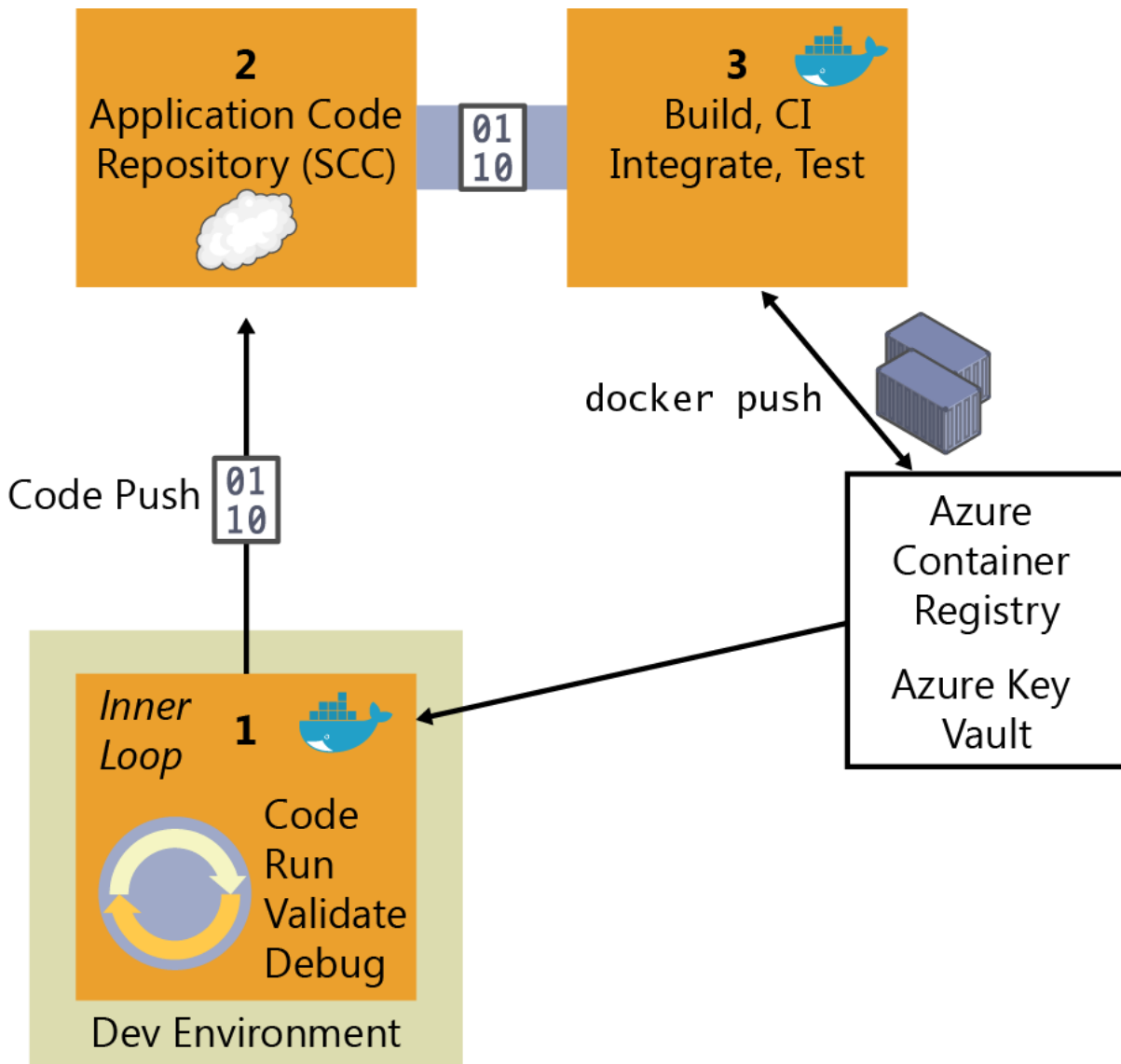
Figure 5-2. The steps involved in CI
