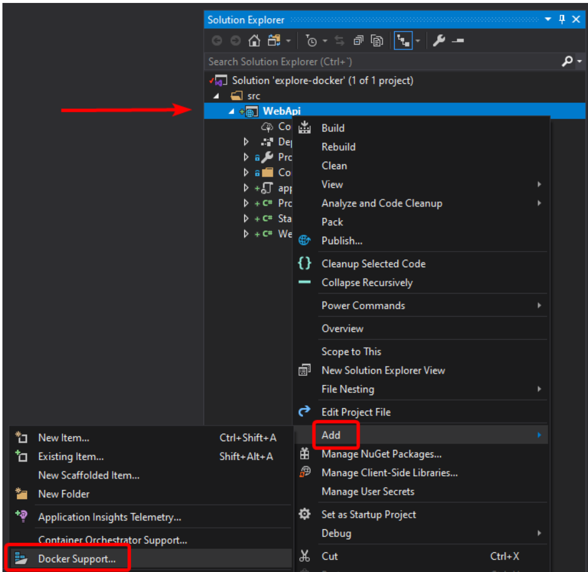
Figure 4-38. Adding Docker support to an existing project
