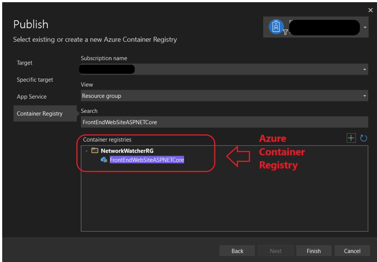
Figure 4-4. Publishing a container to Azure App Service from Visual Studio apps/containers
