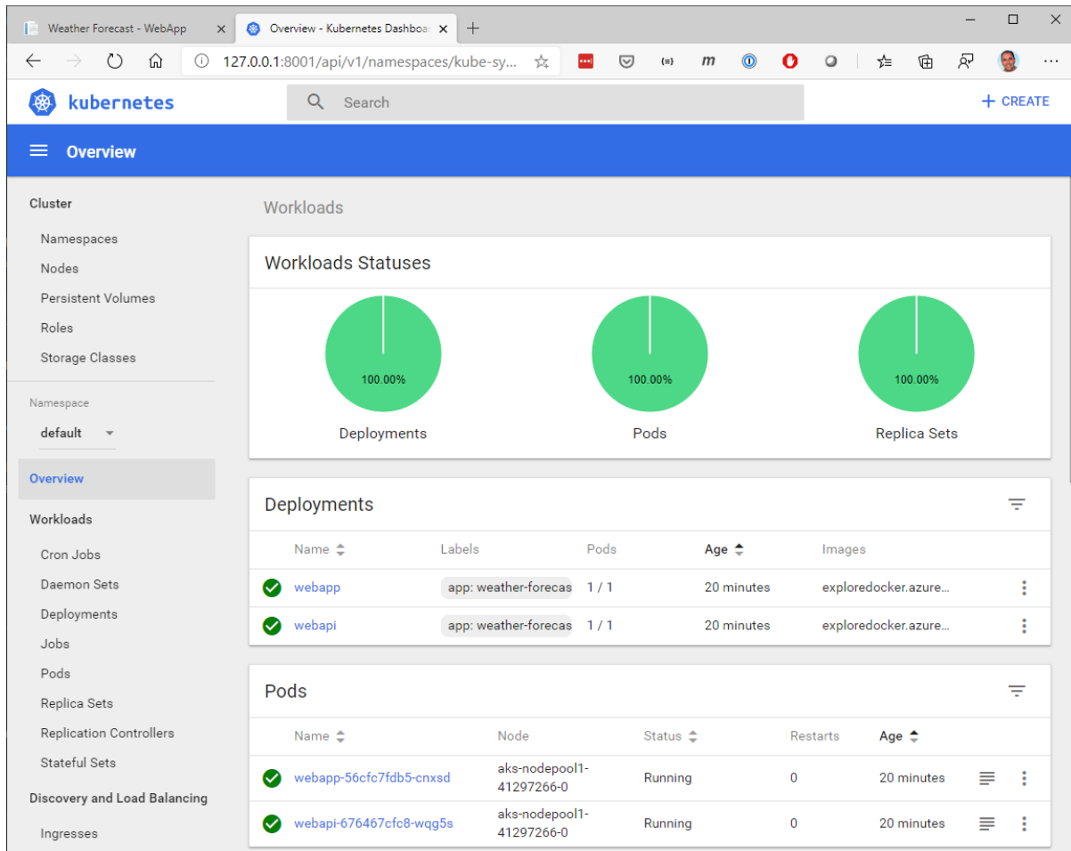
Figure 4-54. View Kubernetes cluster information
