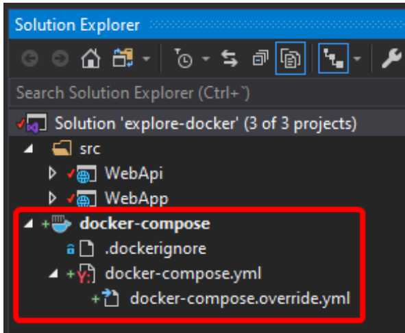
Figure 4-41. Adding orchestrator support to WebApi project.
