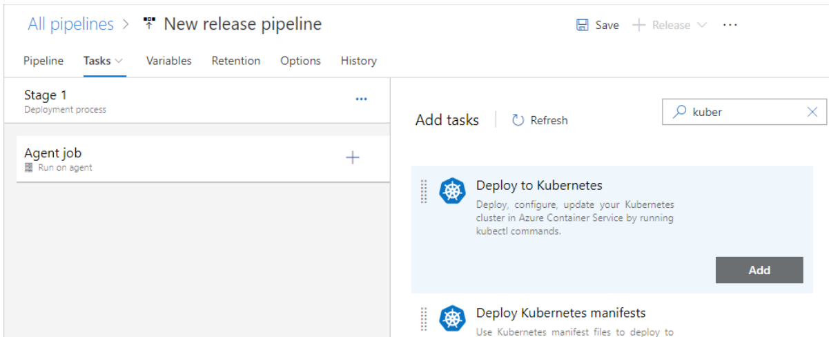
Figure 5-10. Adding the Deploy to Kubernetes task to your Environment
