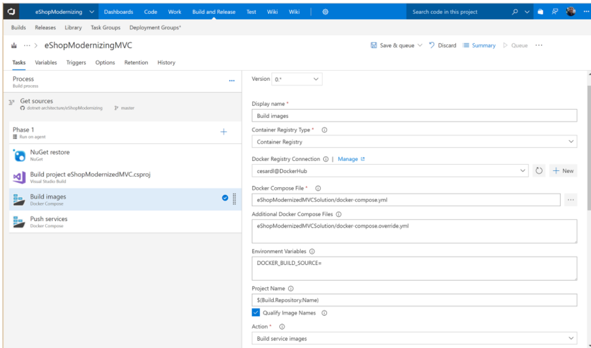
Figure 5-13. Build/CI pipeline in Azure DevOps building Docker images and pushing images to a Docker registry
