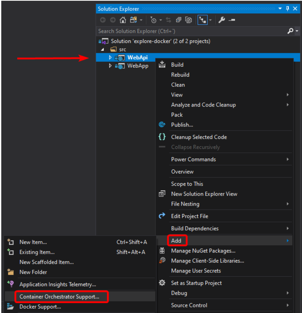
Figure 4-40. Adding orchestrator support to WebApi project.
