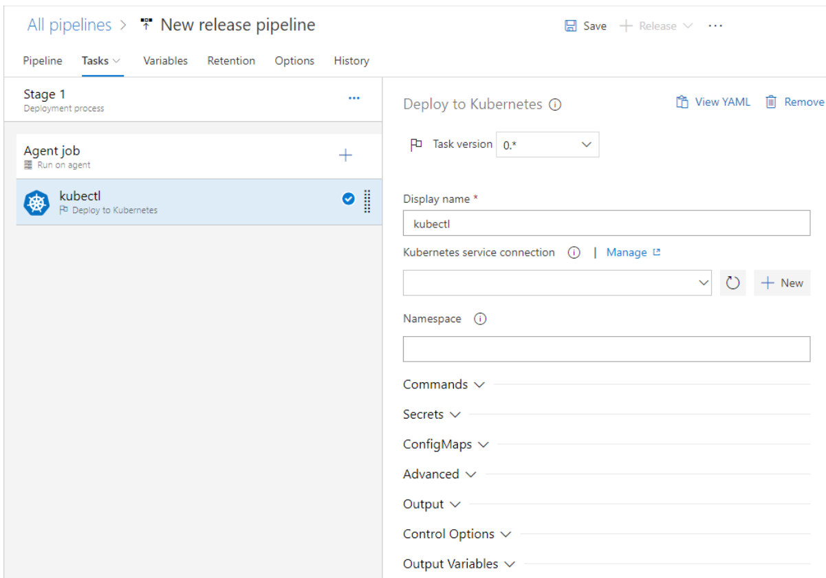
Figure 5-11. Docker Deploy task definition deploying to ACS DC/OS
