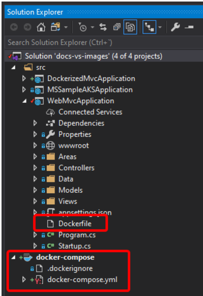
Figure 4-33. Docker files in Solution Explorer in Visual Studio
