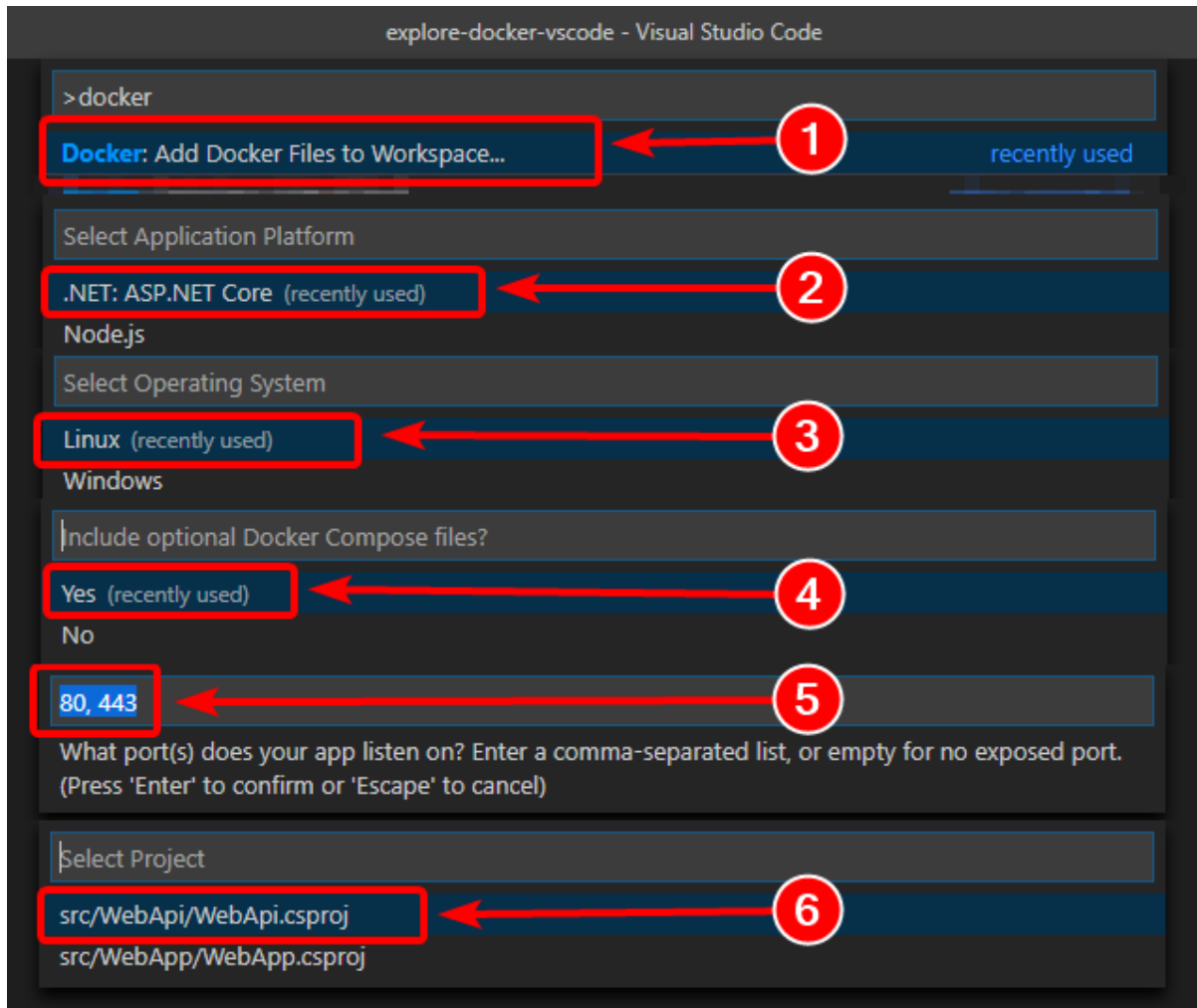
Figure 4-24. Docker files added using the Add Docker files to Workspace command
