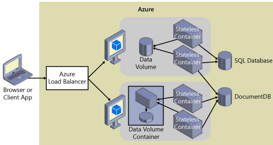
Figure 4-5. Volumes and external data sources for container-based applications
